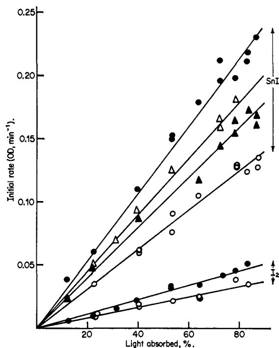
Figure 2. Variation of rate with light absorbed. Light intensities (arbitrary units): \circ , 24; \blacktriangle , 31; \Delta , 34; \bullet , 41.
