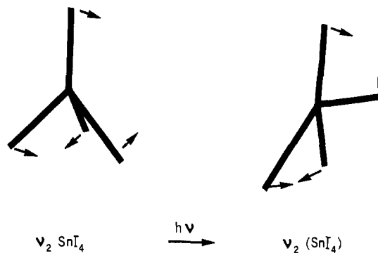
Figure 3. Vibrational model.
