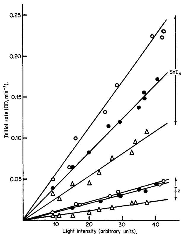
Figure 1. Variation of rate with light intensity. Initial concentration \text{SnI}_4 ( M ): \circ , 1.21 \times 10^{-4} ; \bullet , 0.61 \times 10^{-4} ; \Delta , 0.35 \times 10^{-4} .
